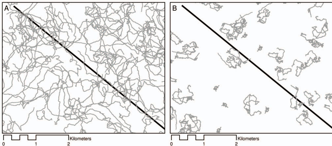
Figure 4. Empirical daily movements dispersed randomly in simulation space. Image capture (1:50 000) shows a single iteration of simulation runs at 2 \text{ km}^{-2} density for (A) gemsbok and (B) steenbok. Approximately half of the randomly oriented transect (black) appears diagonally, underlying travel paths (grey). Note that both gemsbok and steenbok have similar daily travel distances but display different tortuosity in their movements, resulting in different spatial use. doi:10.1371/journal.pone.0096598.g004
