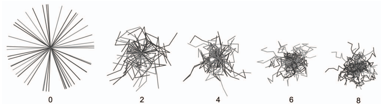
Figure 2. Displacement of simulated animal travel paths over levels of tortuosity. Fifty travel paths of equal length originate from a common centroid for each level of tortuosity (numerals indicate the number of random turn angles). doi:10.1371/journal.pone.0096598.g002
