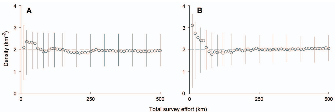
Figure 5. Estimates from simulated densities ( 2 \text{ km}^{-2} ) using empirical movements of (A) gemsbok and (B) steenbok. FMP point estimates of density from a random cumulative increase in survey effort (10 km transects) are displayed along with 95% CIs. doi:10.1371/journal.pone.0096598.g005
