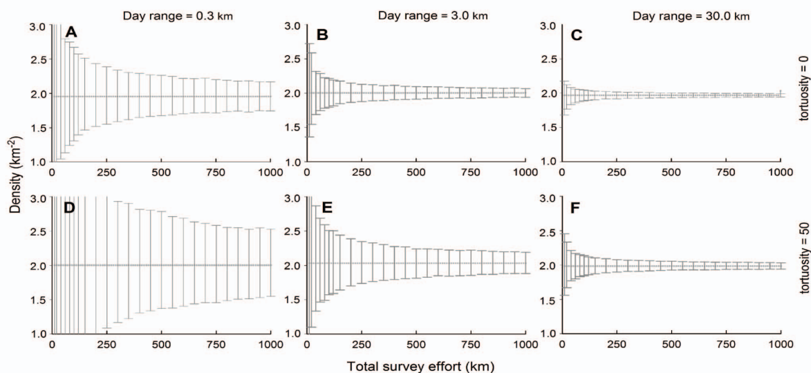
Figure 3. Effect of daily travel distance (column panels) and path tortuosity (row panels) on FMP estimate precision. Mean densities and 95% CIs are shown from applying the FMP formula to 10 km transects sampling virtual populations at 2 \text{ km}^{-2} . Dotted lines indicate the accuracy of mean density estimates at 1200 replicates, which vary within 2% of the true density. Note that both day range and tortuosity influenced achievable precision. doi:10.1371/journal.pone.0096598.g003
