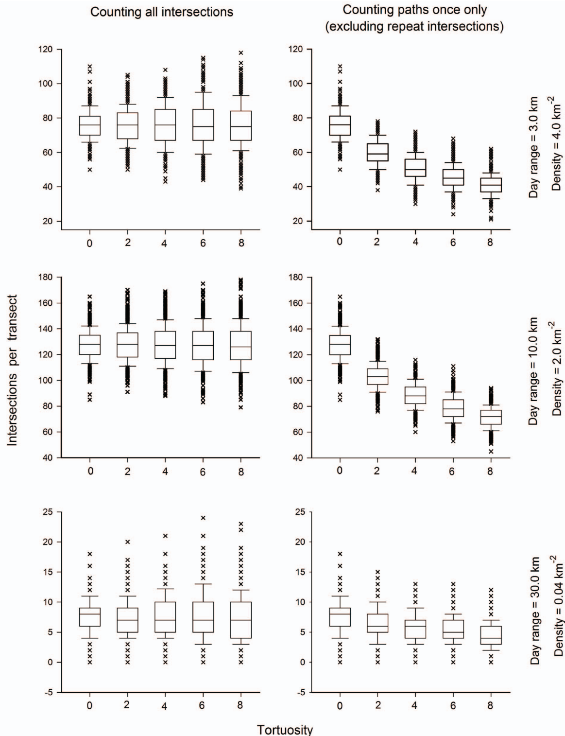
Figure 1. Sample output from three combinations of simulated daily travel paths and densities. Box plots with outliers are shown; each data point represents the numbers of intersections per transect (500 iterations) across five arbitrary levels of travel path tortuosity. doi:10.1371/journal.pone.0096598.g001
