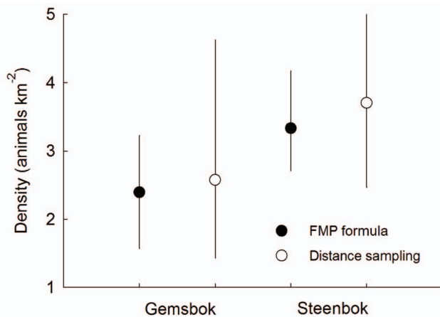
Figure 6. Density estimates of two empirical populations using the FMP formula and Distance sampling. Displayed with 95% bootstrap CIs. doi:10.1371/journal.pone.0096598.g006
